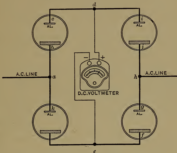
FIG. 23.—THE ELECTROLYTIC CURRENT RECTIFIER.
